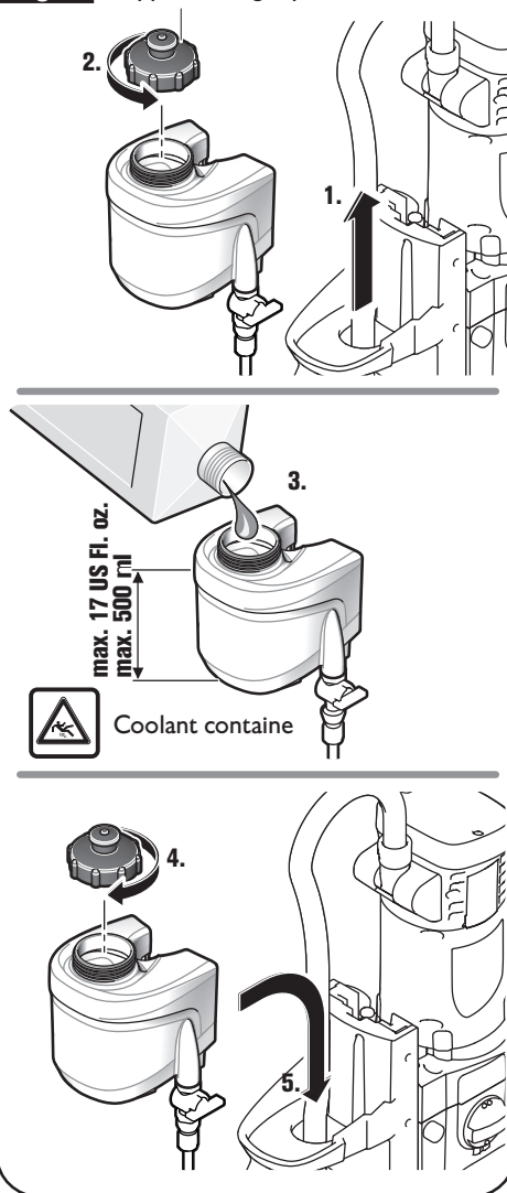
Fig. 4 Upper closing cap
